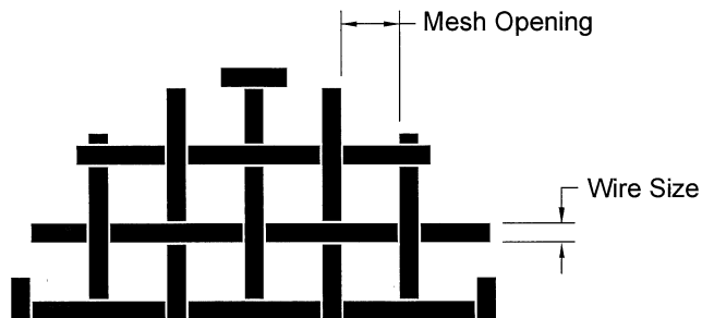
Basket Mesh Detail
